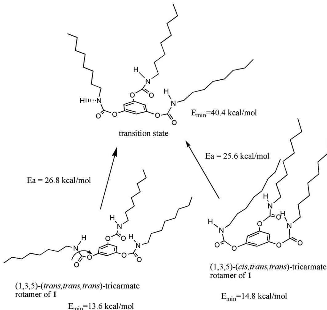
Figure 10. Internal changes between (1,3,5)-( trans, trans, trans )- and (1,3,5)-( cis, trans, trans )-tricarbamate rotamers of inhibitor 1 .
