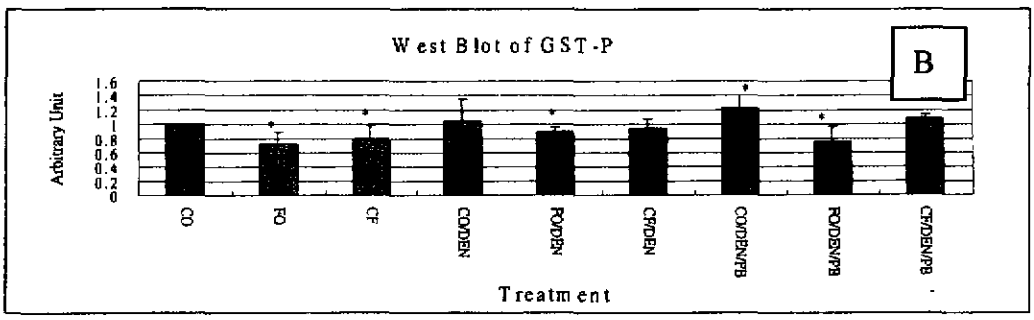
Fig2. Effect of experimental diet on protein expression of rat liver *within the same row are significantly different from CO treatment group (p<0.05). CO (corn oil), FO (fish oil), CF (clofibrate), DEN (diethylnitrosamine), PB (phenobarbital)
