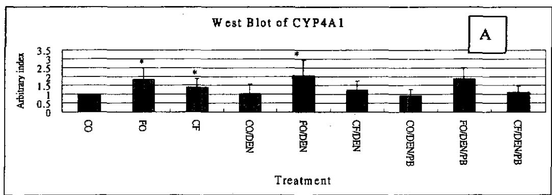
West Blot of CYP4A1
