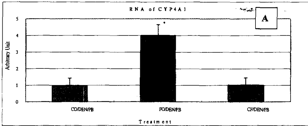
Fig 1. Effect of experimental diet on mRNA expression of rat liver
