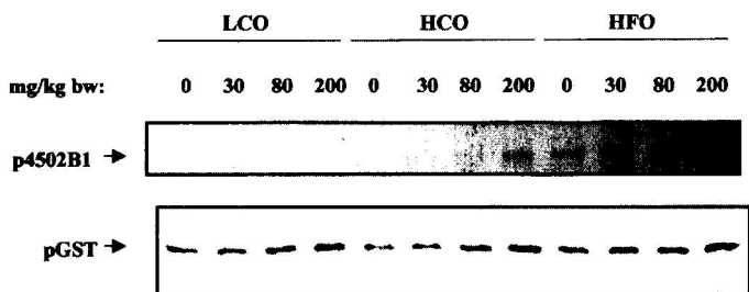
FIGURE 2 Immunoblot analysis of P 450 2B1 and placental glutathione S-transferase (PGST) in rats treated with 0, 30, 80 or 200 mg/kg garlic oil and fed low corn oil (LCO), high corn oil (HCO) or high fish oil (HFO) diets for 6 wk. Proteins were separated on 10% SDS-polyacrylamide gels and electrophoretically transferred to polyvinylidene difluoride membranes. The amount of protein in each lane for P 450 2B1 and PGST immunostaining was 6 and 3 \mu g, respectively. Protein level was quantitated by densitometry and the value in rats fed the LCO diet and receiving no garlic oil was regarded as 1.0. A representative experiment is shown. The average fold inductions of P 450 2B1 of three separate experiments were (from left to right) 1.0 \pm 0 , 1.50 \pm 0.36 , 1.91 \pm 0.36 , 3.98 \pm 0.37 , 1.75 \pm 0.77 , 3.29 \pm 0.96 , 4.33 \pm 1.99 , 6.99 \pm 1.72 , 5.70 \pm 1.46 , 10.0 \pm 3.80 , 9.60 \pm 3.20 , 14.3 \pm 5.19 , respectively, and those of PGST were 1.0 \pm 0 , 1.43 \pm 0.19 , 1.46 \pm 0.14 , 1.76 \pm 0.35 , 1.03 \pm 0.18 , 1.23 \pm 0.20 , 1.56 \pm 0.17 , 1.69 \pm 0.23 , 1.33 \pm 0.19 , 1.71 \pm 0.38 , 1.94 \pm 0.21 , 2.30 \pm 0.40 , respectively.
