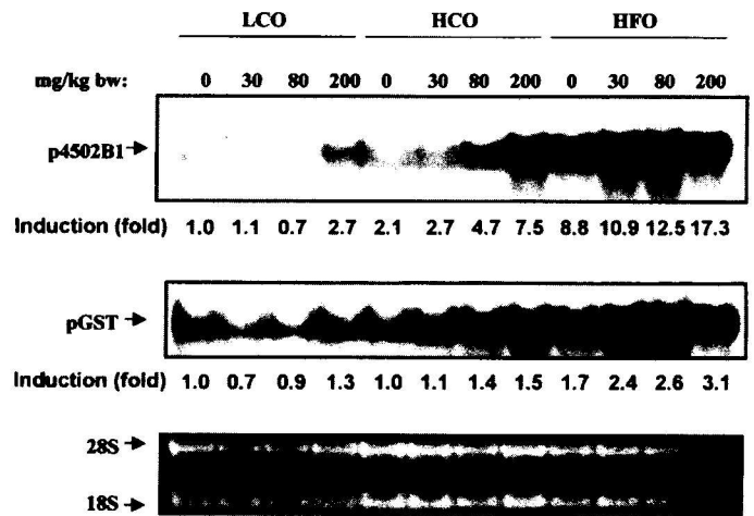
FIGURE 1 Hepatic P 450 2B1 and placental glutathione S-transferase (PGST) mRNA level in rats fed low corn oil (LCO), high corn oil (HCO) or high fish oil (HFO) diets and treated with 0, 30, 80 or 200 mg/kg garlic oil for 6 wk. Total RNA was extracted by Trizol as described in Materials and Methods. An equal amount of RNA was subjected to Northern blot analysis (20 µg/lane). The filter was first hybridized with a P 450 2B1 cDNA and then rehybridized with a PGST cDNA after deprobing. The fold of induction was quantitated by densitometry based on the relative amount of 18S RNA. A representative experiment is shown. The average values of P 450 2B1 mRNA induction of three separate experiments were (from left to right) 1.0 ± 0, 1.47 ± 0.57, 1.92 ± 1.07, 3.39 ± 0.70, 1.54 ± 0.55, 2.24 ± 0.40, 3.63 ± 1.00, 9.96 ± 2.91, 7.17 ± 3.20, 9.07 ± 3.33, 14.06 ± 1.65, 17.91 ± 2.06, respectively, and those of PGST mRNA were 1.0 ± 0, 0.93 ± 0.31, 1.48 ± 0.52, 2.05 ± 0.93, 1.08 ± 0.41, 1.38 ± 0.51, 1.76 ± 0.37, 1.98 ± 0.65, 1.88 ± 0.41, 2.65 ± 0.84, 2.70 ± 0.63, 3.61 ± 1.0, respectively.
