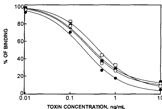
Figure 3. Cross-reactivity of anti-MCYST antibodies with MCYST-LR (●) MCYST-RR(O), MCYST-YR(■), and Nodularin(□) as determined by an competitive indirect ELISA(ciELISA).
